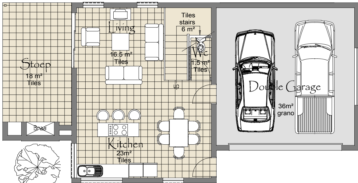
1:100 Unit A1 - Ground Floor Plan
