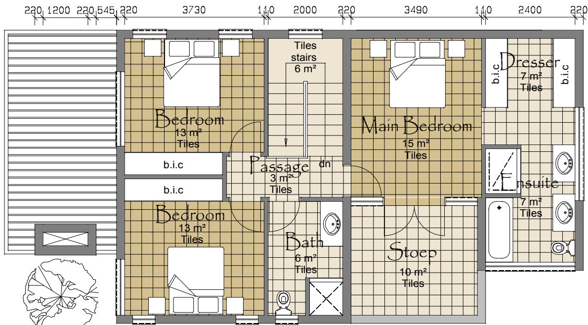
1:100 Unit A1 - First Floor Plan
