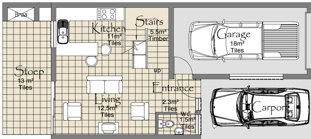
1:100 Unit B- Ground Floor Plan
