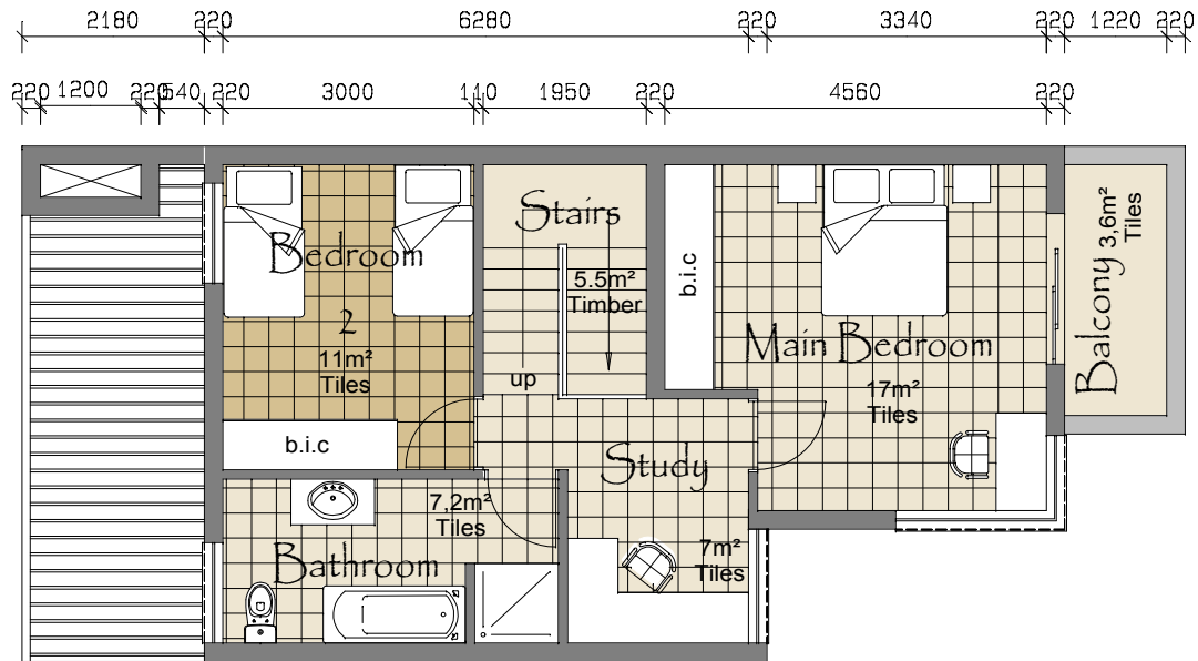
1:100 Unit B- First Floor Plan
