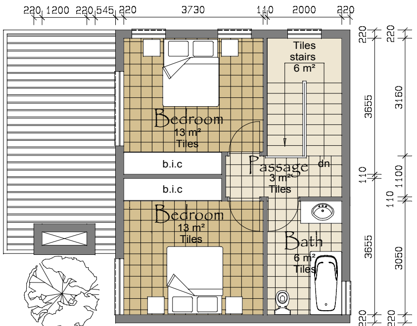
1:100 Unit A2, A4, A6 & A7 - First Floor Plan
